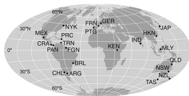
Figure 1 Location of study sites on six continents (ARG, Argentina; NSW, Australia-New South Wales; QLD, Australia-Queensland; TAS, Australia-Tasmania; BRL, Brazil; CHL, Chile; HKN, China-Hong Kong; CRA, Costa Rica; FRN, France; FGN, French Guiana; GER, Germany; IND, India; JAP, Japan; KEN, Kenya; MLY, Malaysia; MEX, Mexico; NZL, New Zealand; PAN, Panama; PTG, Portugal; PRC, Puerto Rico; TRN, Trinidad; NYK, USA-New York).
