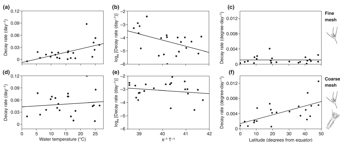
Figure 2 Variation in decomposition rates of litter in fine-mesh (a, b, c) and coarse-mesh bags (d, e, f) across 22 globally distributed study sites. Relationships between decomposition coefficients and stream temperature in ^{\circ}\text{C} (a, d), between the natural logarithm of decay rate coefficients per day and stream temperature expressed in the terms of metabolic theory of ecology (MTE) as the inverse of absolute temperature ( T ) in Kelvin and the Boltzmann constant ( k ) in \text{eV}/k (b, e) and between temperature-normalized decay coefficients per degree day with latitude (c, f). Icons represent a spore of an aquatic fungal decomposer (drawing: E. Chauvet) and a litter-consuming caddisfly larva (drawing: A. Cairns, with permission).
